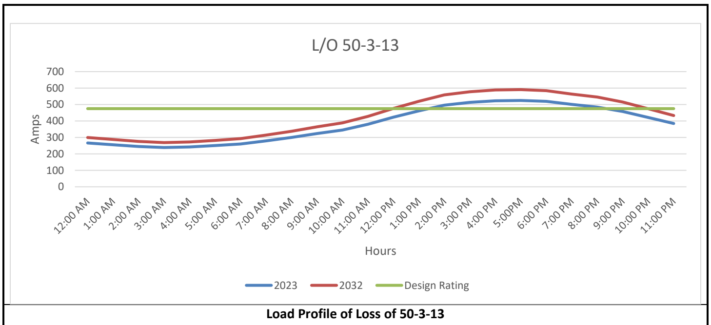
Figure 2: Load profile for the Loss of Circuit 50-3-13 on a peak day
