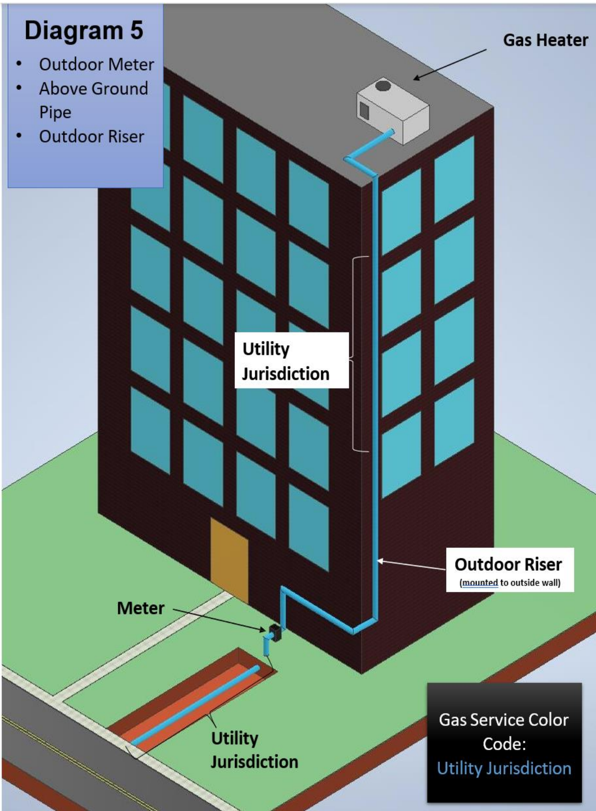
Note: The purpose of the diagram is to depict the jurisdiction of Gas Service Line vs. Customer Piping.
