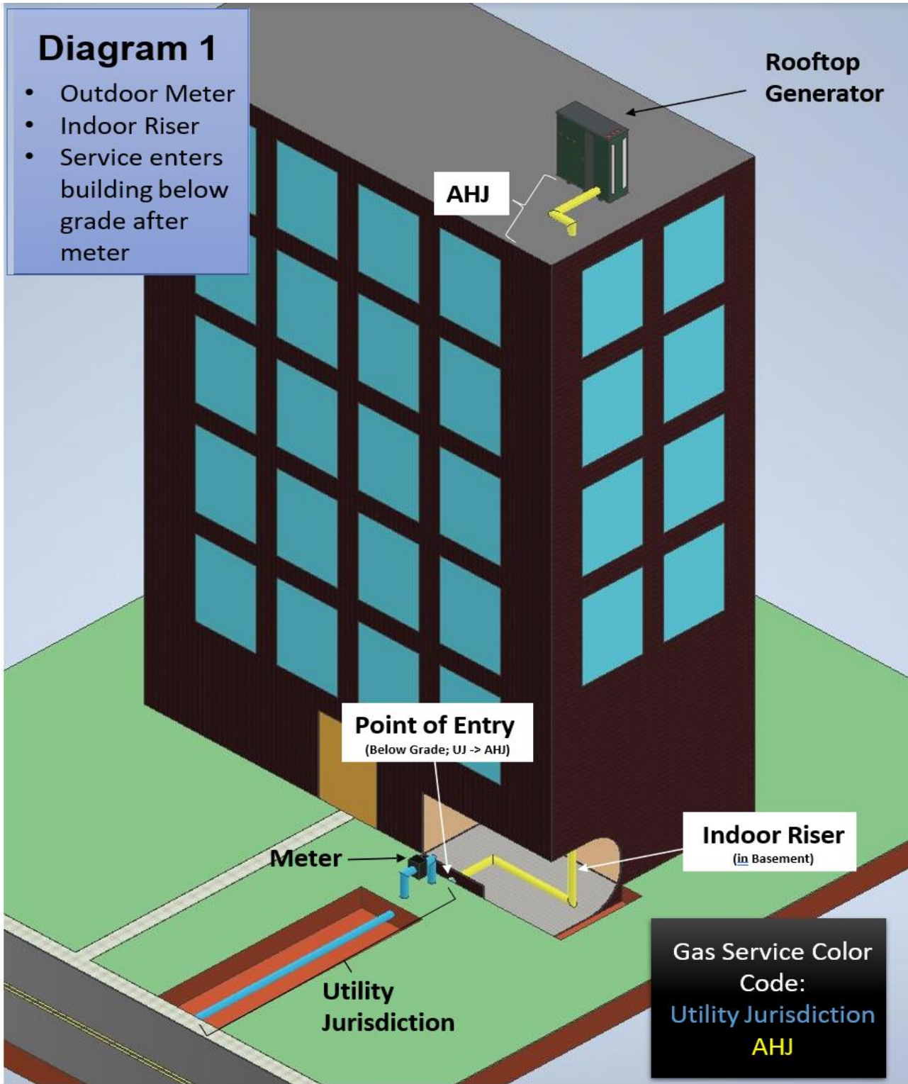
Note: The purpose of the diagram is to depict the jurisdiction of Gas Service Line vs. Customer Piping.
