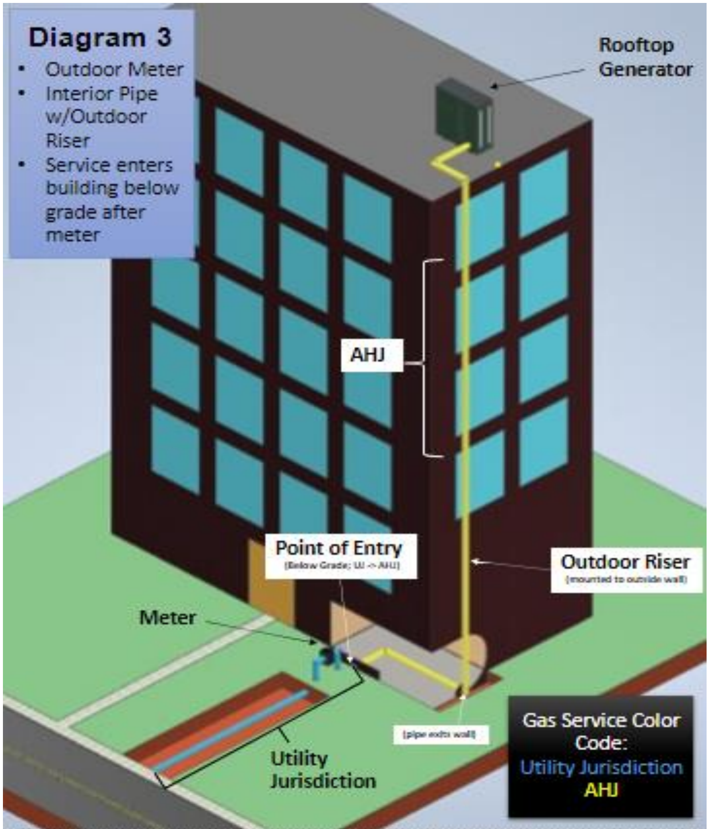
Note: The purpose of the diagram is to depict the jurisdiction of Gas Service Line vs. Customer Piping.
