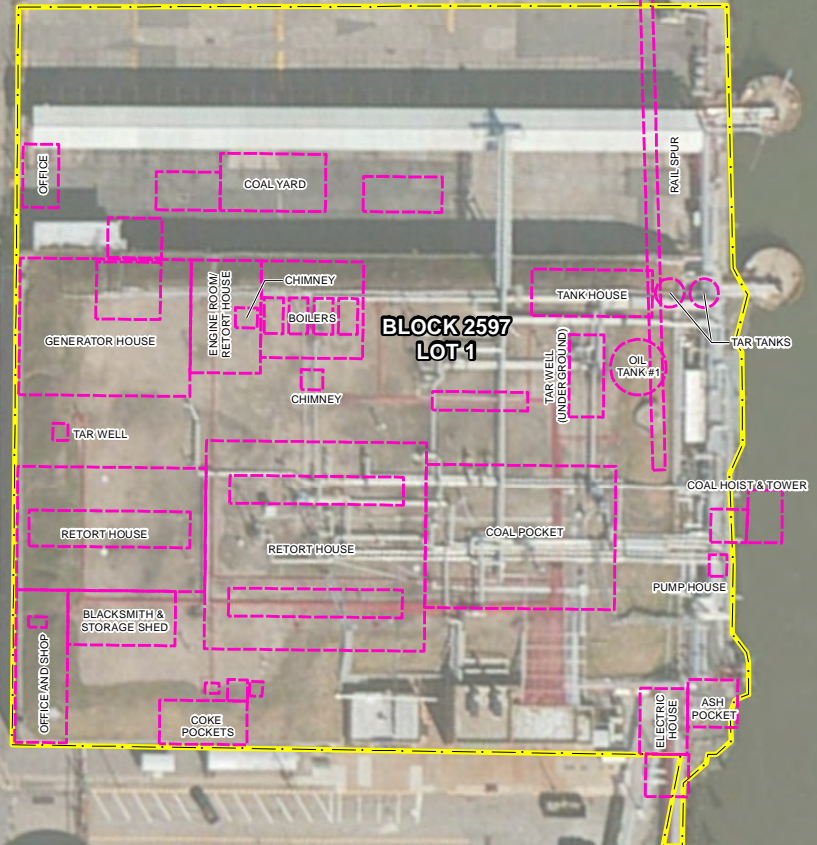
EAST 138TH STREET WORKS SITE FORMER MGP SITE PLAN FIGURE 2
